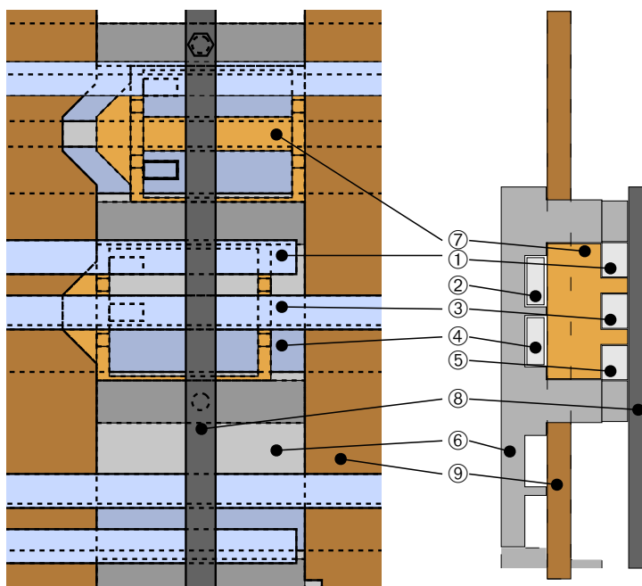
Figure 1: A section through a 5-bar locking tray has been marked up to show the bars, locking nibs and tappet. A lock of solid construction is fixed to a single bar whereas a hollow lock can be driven by several bars. On the left hand view, 'V'-shaped notches may be seen, cut into the tappets. A plate or a condition piece may be mounted on a tappet to engage with the upper half of a lock (or with a 'top thin' lock). Locking bars ① to ⑤, the tray ⑥, a sliding lock ⑦, strap ⑧ and tappet ⑨ are labelled.
