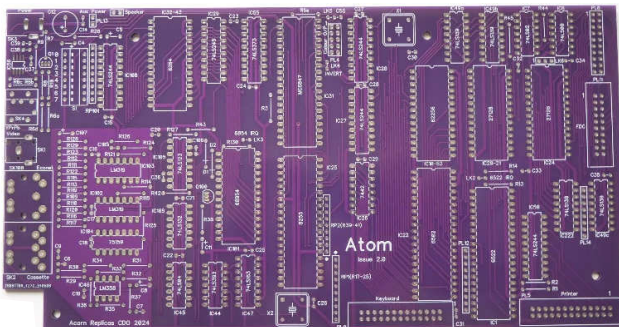
The bare replica Atom PCB
